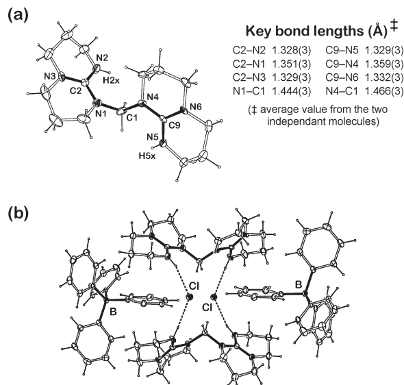
Fig. 3 (a) ORTEP of one of the cationic components of 3b (ellipsoids drawn at 30%). (b) Dimeric arrangement of [H 2 C{hppH} 2 ][Cl][BPh 4 ] showing NH···Cl hydrogen bonds.
